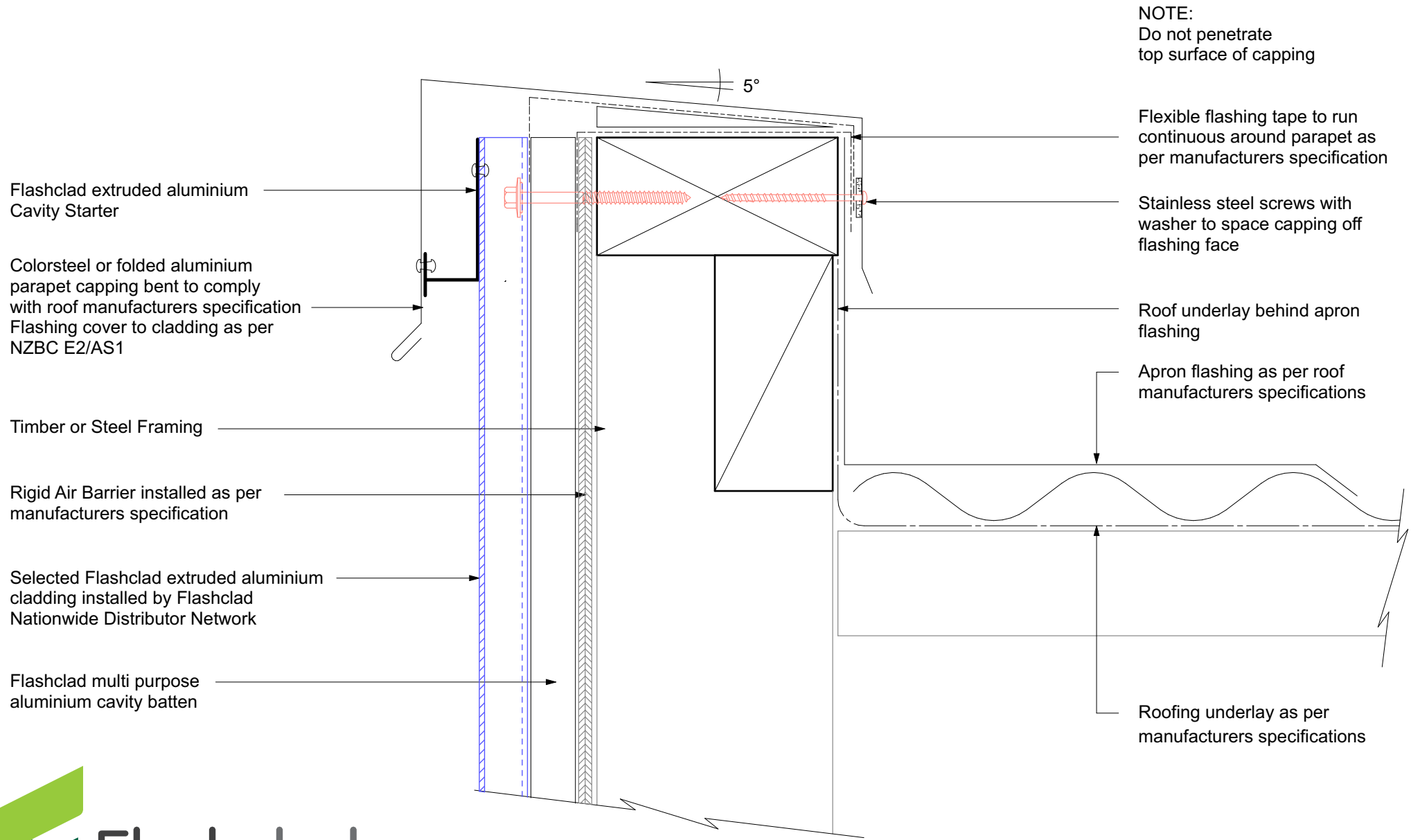
PARAPET CAP Original Scale 1:2 Revision - 01 October 2019
