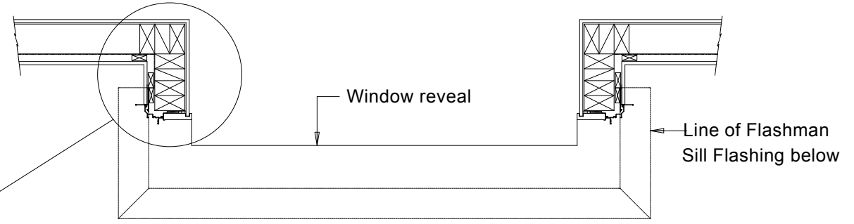
BOX WINDOW PLAN
