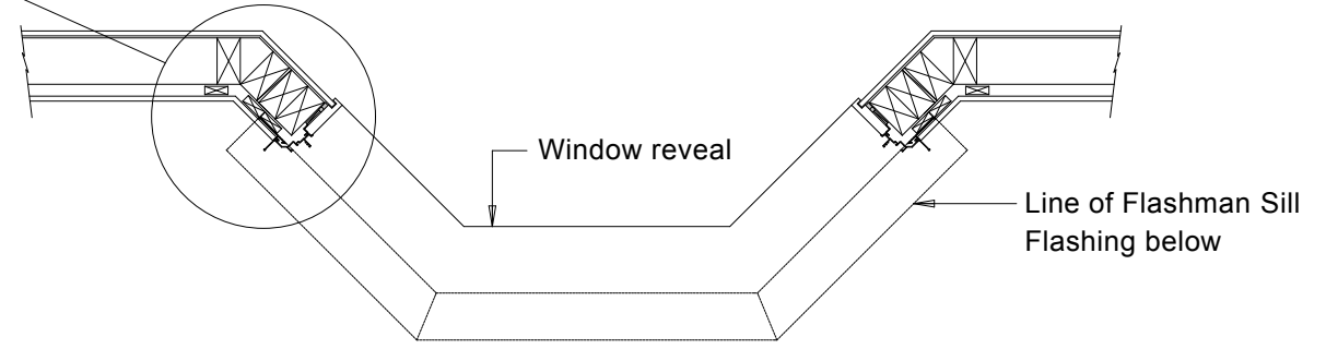
BAY WINDOW PLAN
